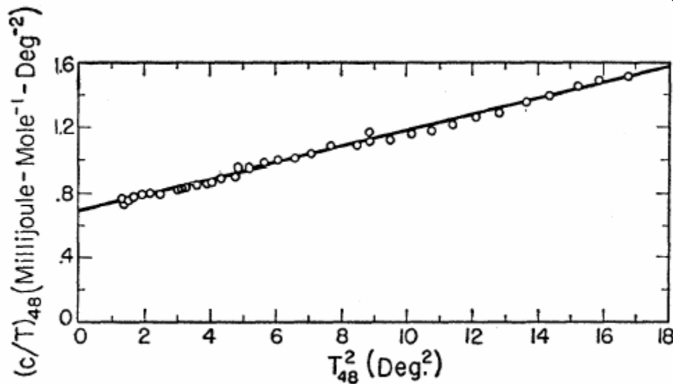
FIG. 5. Atomic heat of copper.
