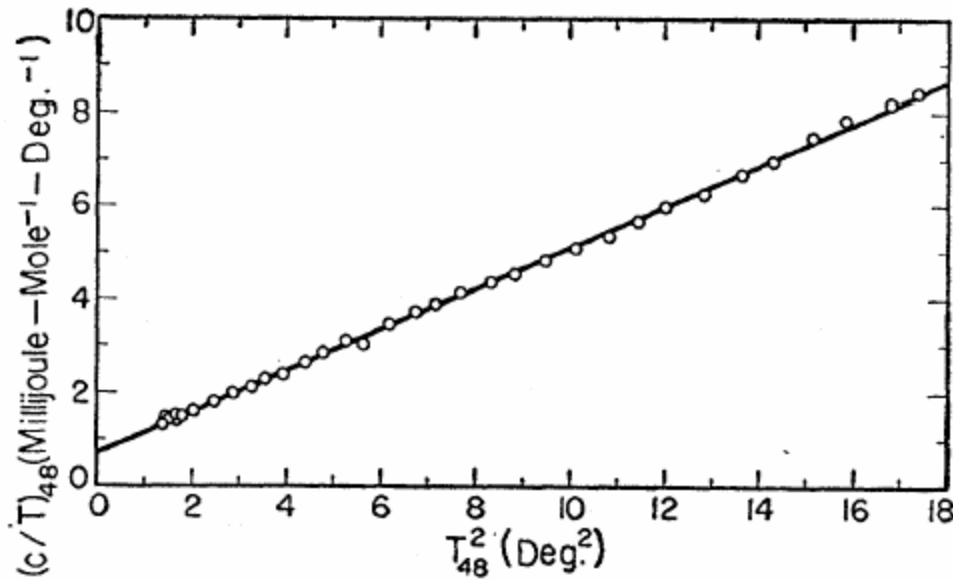
FIG. 7. Atomic heat of gold.
