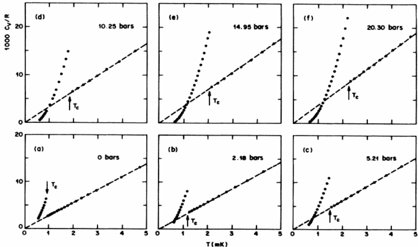
Measurement of the heat capacity of helium-3
