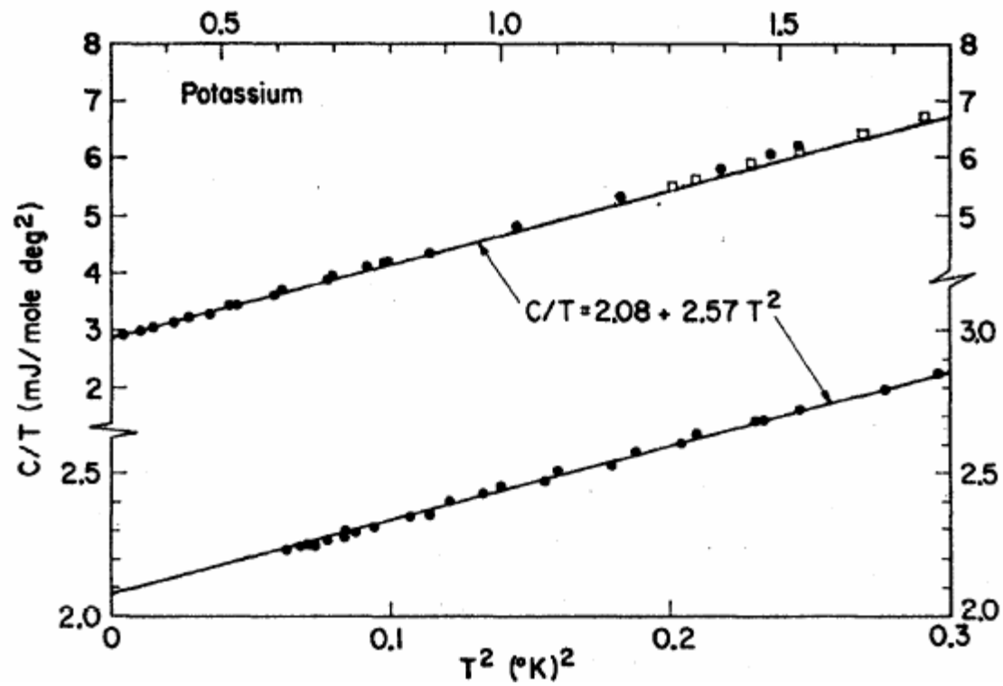
Measurement of the heat capacity of potassium
